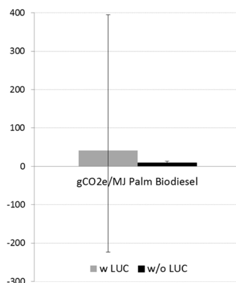
Fig. 3. Comparison of LCA results on palm biodiesel (PME) based on collected data In [4] : mean GHG balance per MJ of palm biodiesel (PME) and minimum and maximum values with and without considering land use change (LUC)
