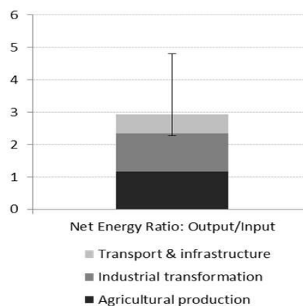
Fig. 2. Comparison of LCA results on palm biodiesel (PME) based on collected data In [4]: mean Net Energy Ratio and minimum and maximum values
